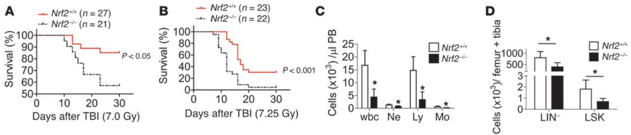
Figure 3 NRF2-null mice show increased sensitivity to TBI-induced mortality and myelosuppression. (A and B) Thirty-day survival rate of Nrf2^{-/-} and Nrf2^{+/+} mice exposed to (A) 7.0 Gy and (B) 7.25 Gy TBI. (C and D) Differential blood counts (C) (wbc, neutrophils [Ne], lymphocytes [Ly], and monocytes [Mo]) and LSK cell populations (D) in Nrf2^{+/+} and Nrf2^{-/-} mice on day 23 after TBI (6.9 Gy). * P < 0.05 compared with Nrf2^{-/-} mice.
