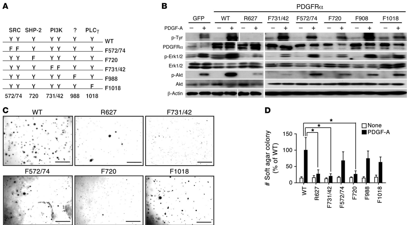
Figure 5 Impacts of PDGFR \alpha mutations on downstream signaling of PDGFR \alpha and anchorage-independent growth in soft agar of Ink4a/Arf -/- mAst cells. (A) Schematics of various PDGFR \alpha mutants. (B) IB analyses of PDGF-A-stimulated Ink4a/Arf -/- mAst cells overexpressing individual PDGFR \alpha mutants. Corresponding total proteins or \beta -actin were used as loading controls. Vertical lines in left panels of p-Tyr, PDGFR \alpha , and \beta -actin indicate that these images were modified by removal of two lanes of samples between WT and R627. The longer white vertical line indicates that the samples were analyzed in separate SDS-PAGE gels due to the limit of sample loading per gel. (C and D) Soft agar assay. (C) Representative images of soft agar colonies. (D) Quantification of soft agar assays. Data are presented as mean \pm SD and are representative of 2 independent experiments. Scale bars: 1 mm. * P < 0.01.
